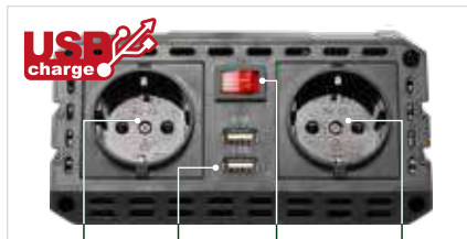
USB charge Schuko USB: 5V-3,1A On / Off Schuko
